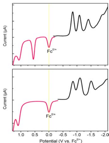
Figure 2. Differential pulse voltammograms of \text{Lu}_3\text{N}@I_h\text{-C}_{80}\text{-PDI} ( 6 ) (up) and \text{C}_{60}\text{-PDI} ( 7 ) in o -dichlorobenzene (0.05 M ( n -Bu) 4 NPF 6 with ferrocene as internal standard, scan rate: 20 mV s −1 ).
