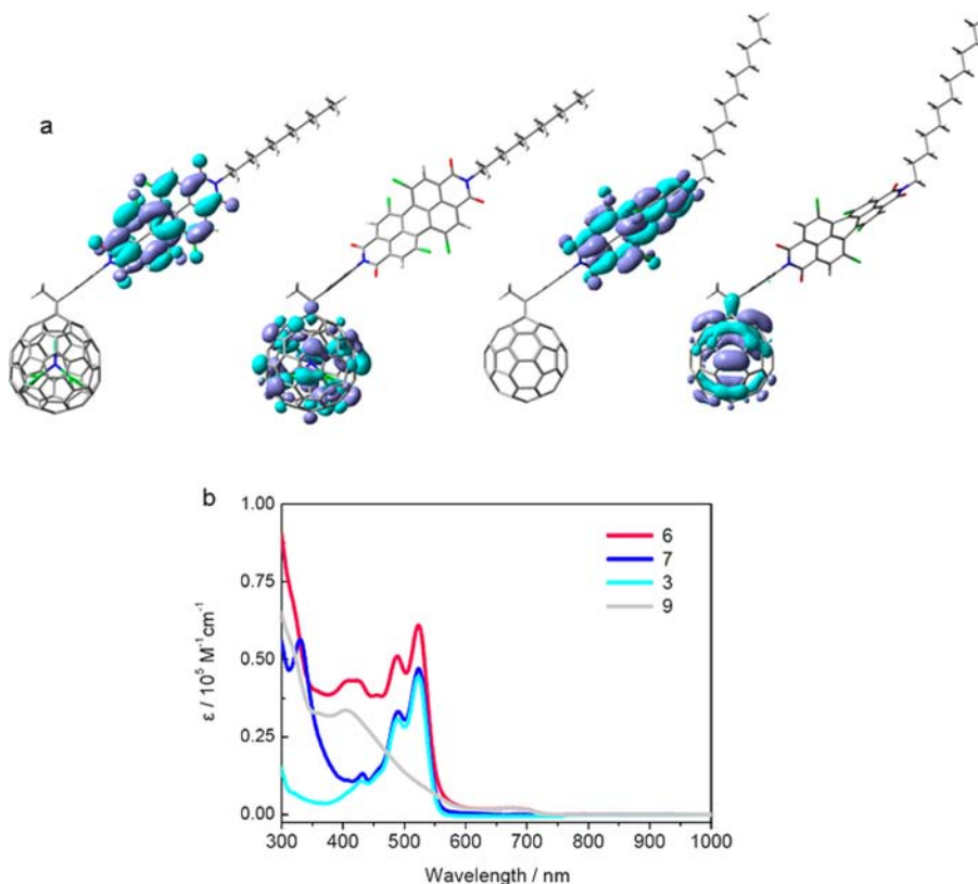
Figure 3. (a) LUMO/HOMO distributions of Lu 3 N@I h -C 80 -PDI (6) (left panel) and C 60 -PDI (7) (right panel) at the M06-2X/3-21G~SDD level; (b) Absorption spectra of 6 ( \epsilon_{\max} : 61010), 7 ( \epsilon_{\max} : 47050), PDI-ref (3) ( \epsilon_{\max} : 44770), and Lu 3 N@C 80 -ref (9) in toluene at 298 K.
